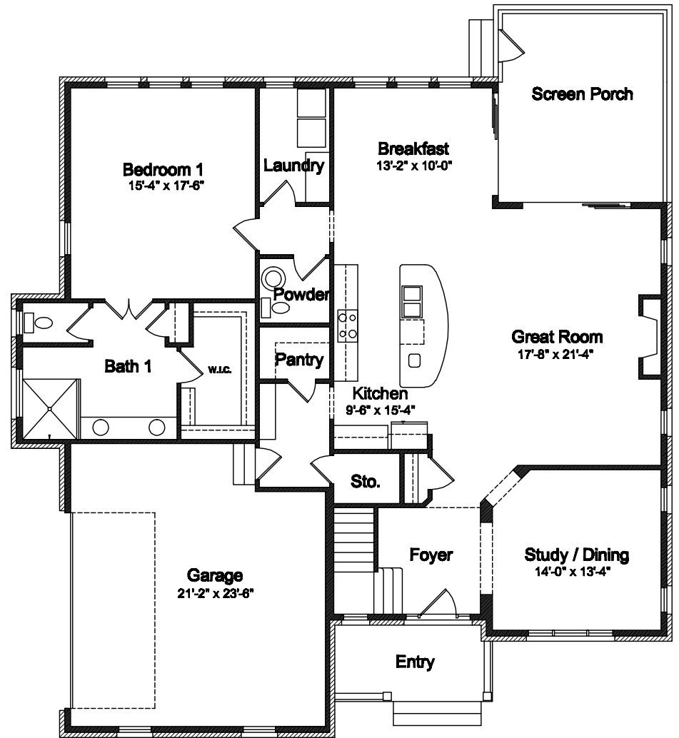
First Floor 1867 s.f.
