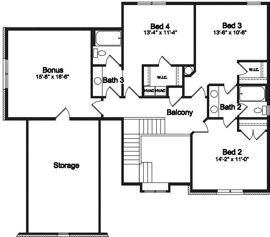
Second Floor 1254 s.f.
